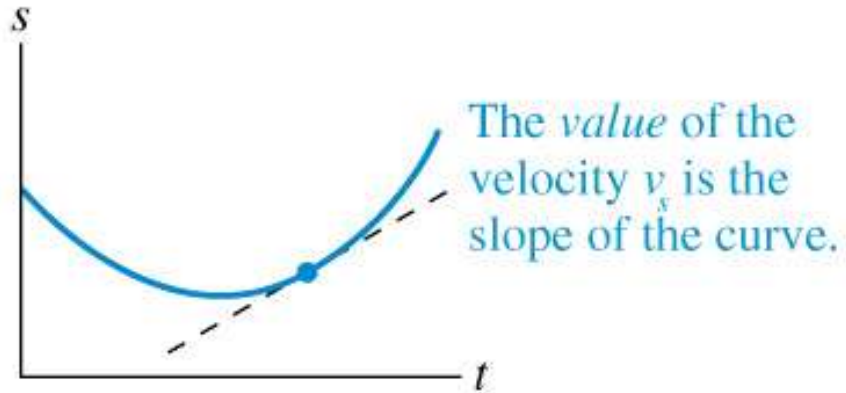
Position-versus-time graph
