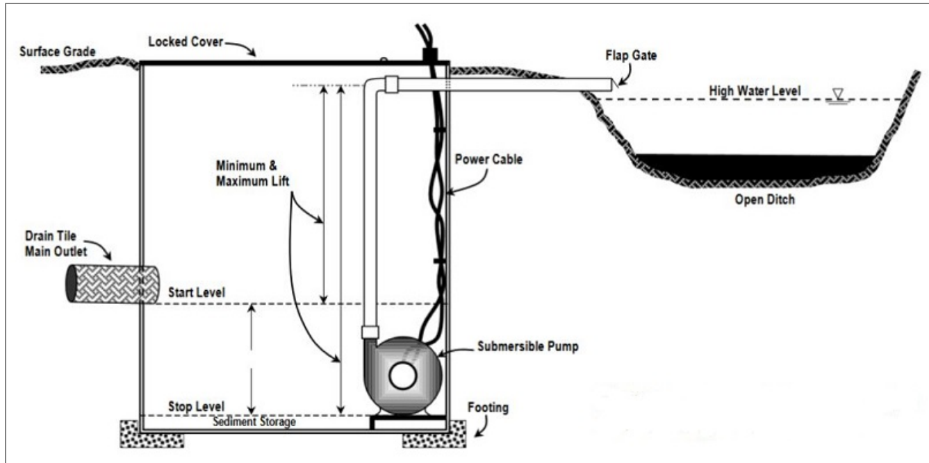
Figure 2. A simple drainage pump station using a submersible pump.
